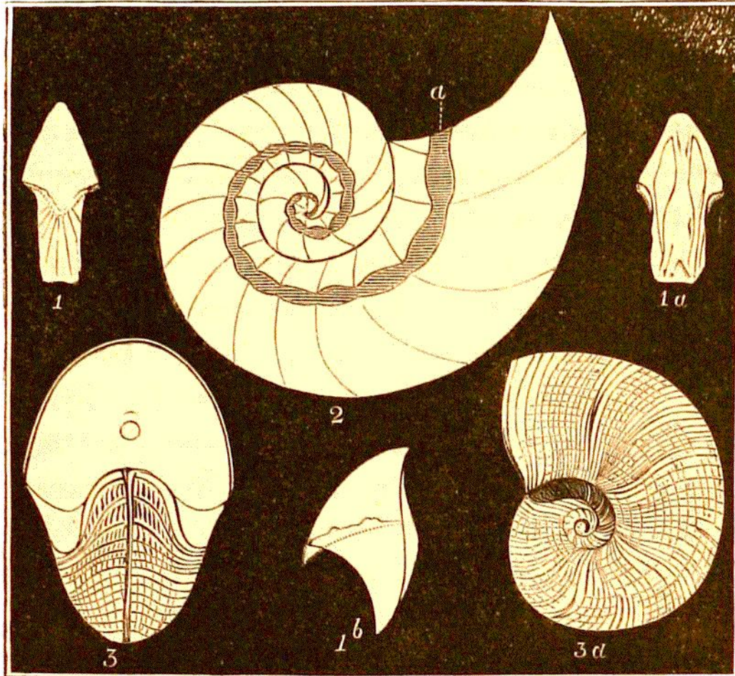
LIGN. 105. FOSSIL NAUTILI. Chalk-marl.
