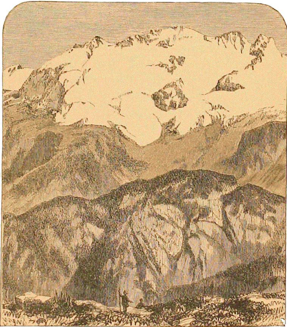
FIG. 114.—GLACIER OF THE MALADETTA (PYRENEES). (From a Photograph by Ferrier.)
