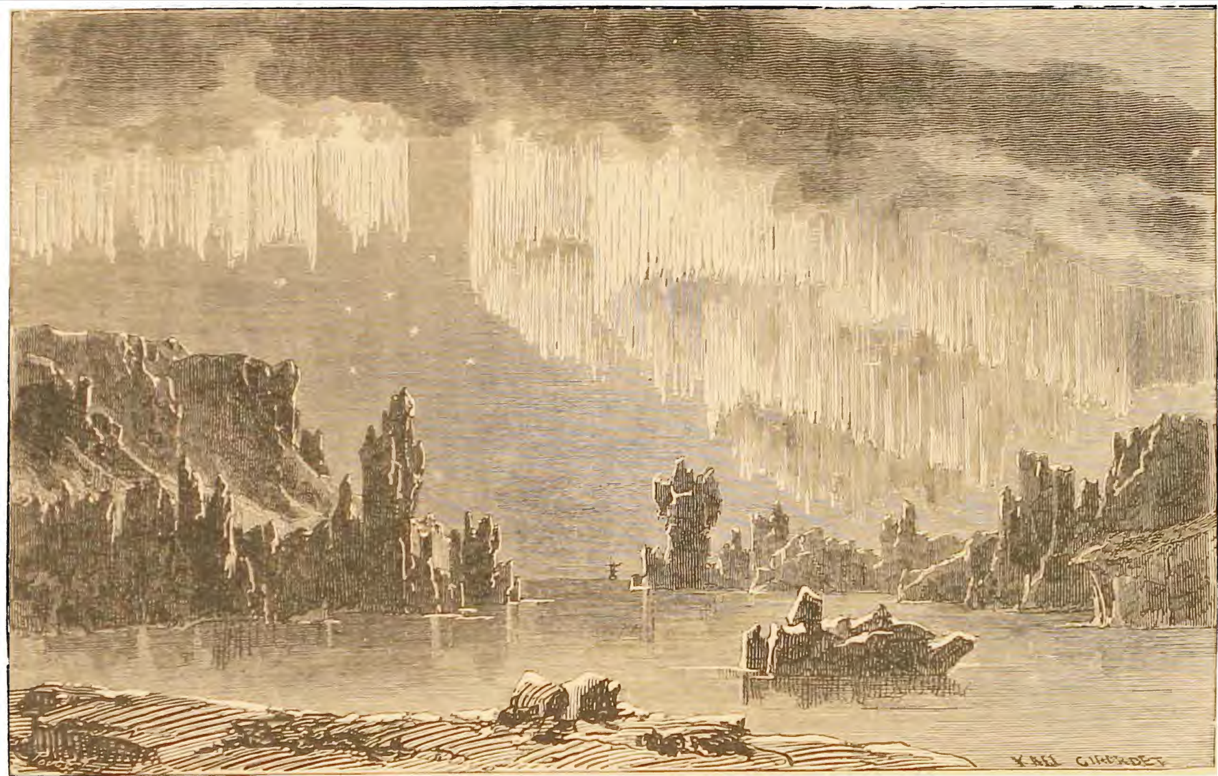
FIG. 232. AURORA BOREALIS IN THE ARCTIC SEAS.
