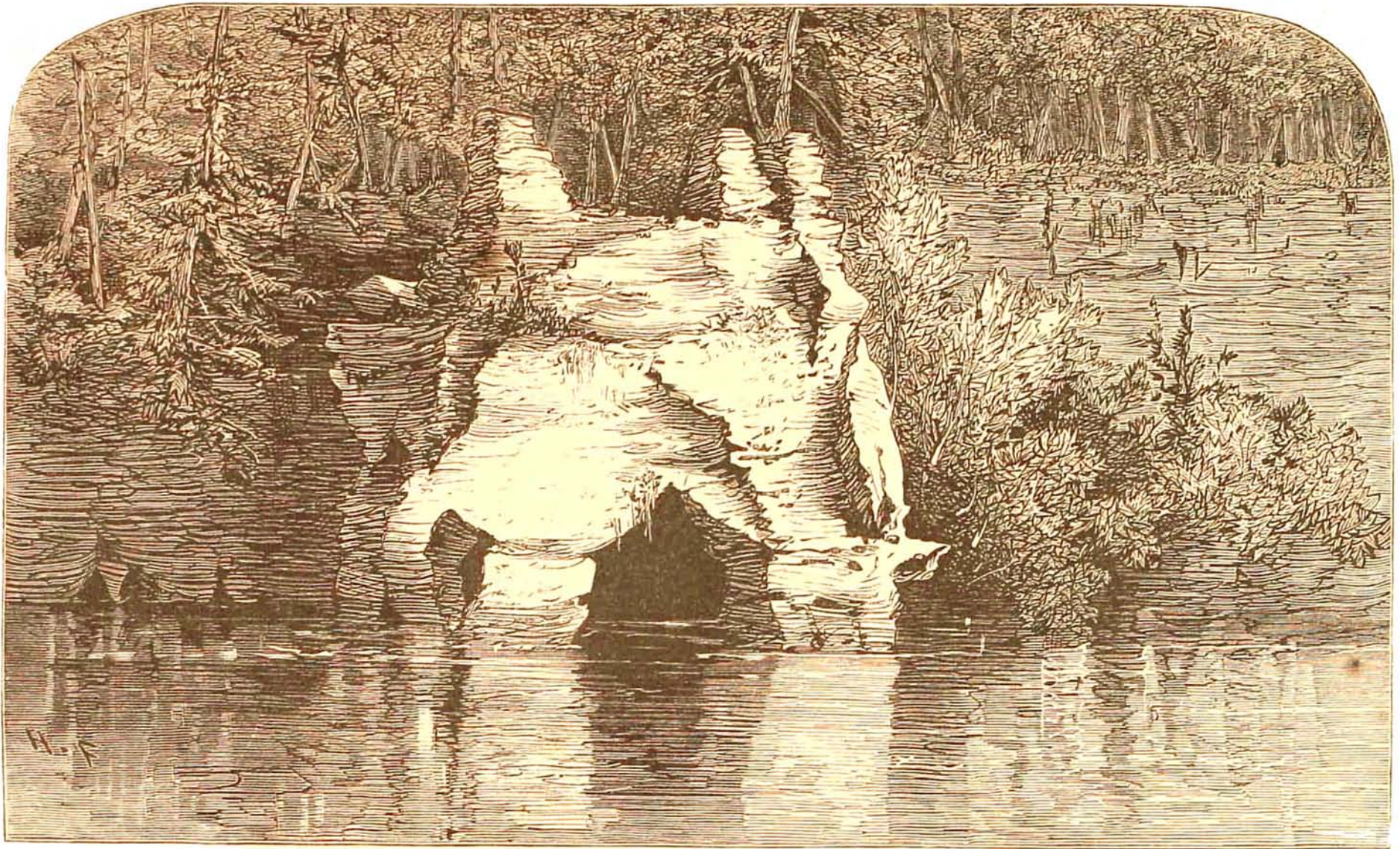
Fig. 32. The Miners' Castle—"Pictured Rocks," Lake Superior.
