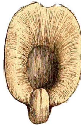
Bellerophon dilatatus.
