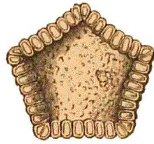
Goniaster Coombii
