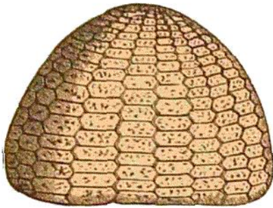
Ananchites ovatus.
