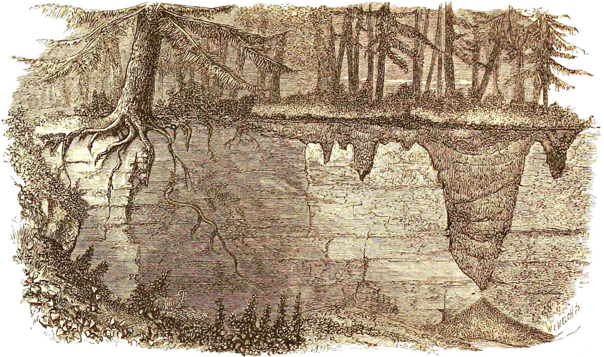
Potholes in the Chalk of Savernake Forest, near Marlborough.
