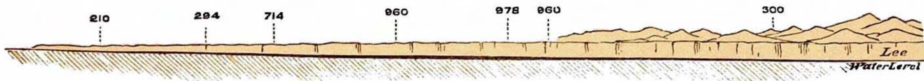
FIG. 93. Old Glacier of the Rhone, covering what is now the Lake of Geneva.
