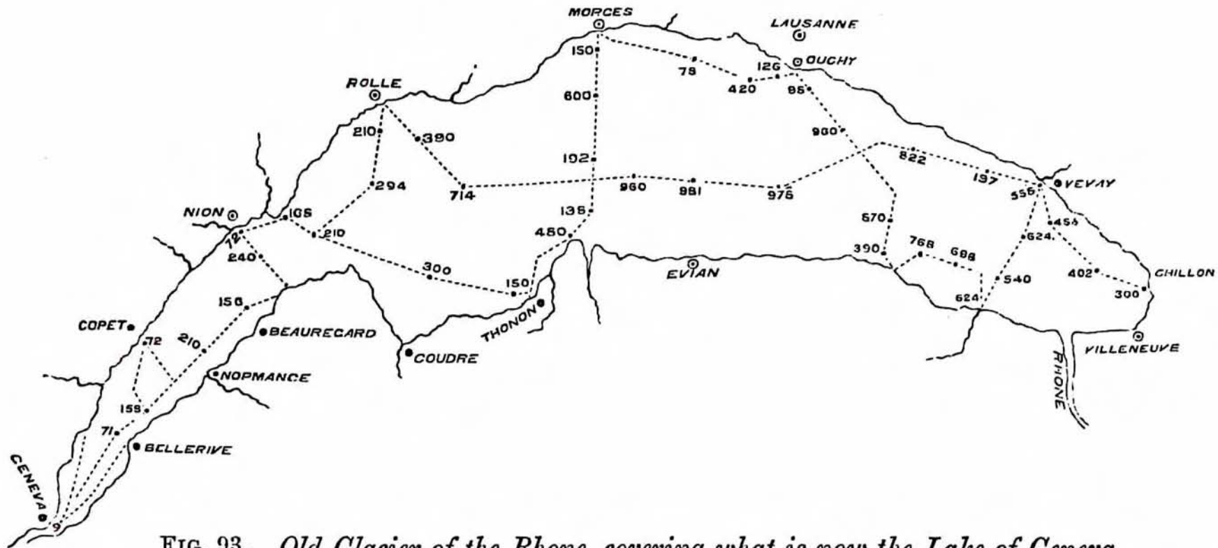
FIG. 93. Old Glacier of the Rhone, covering what is now the Lake of Geneva.
