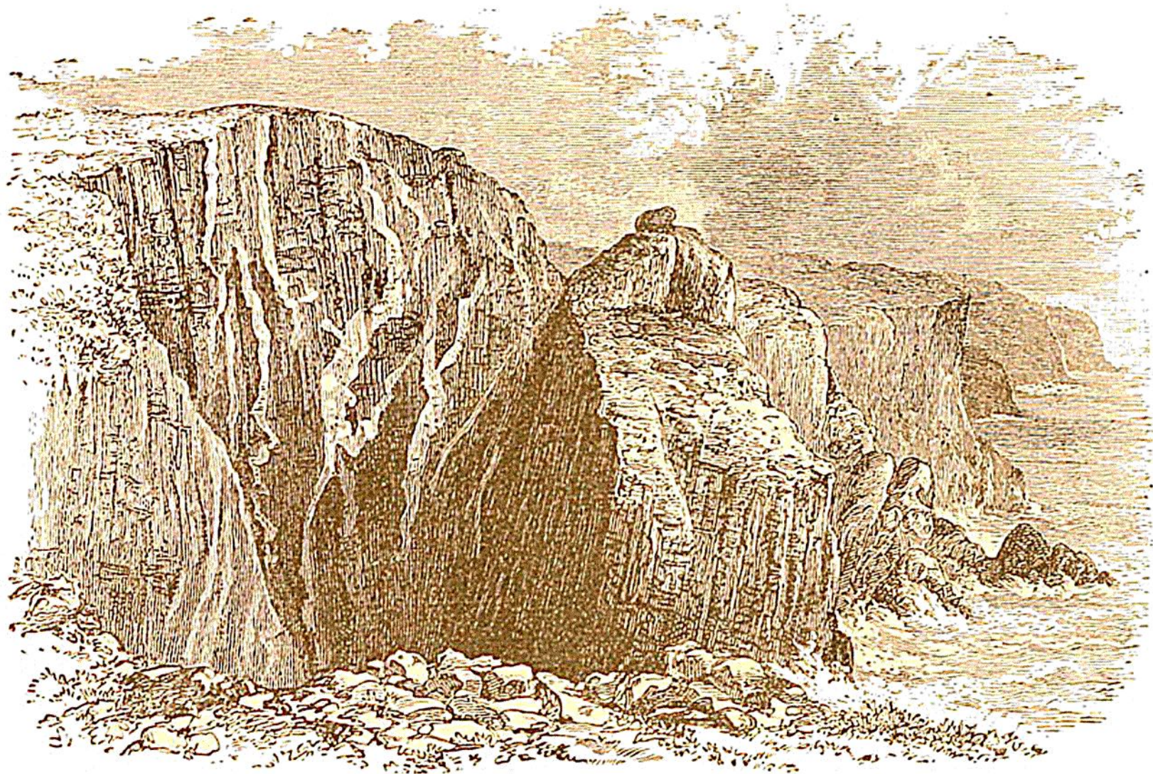
Fig. 4.—View of the Gneiss Cliffs near Cape Wrath, with tortuous granitic veins.
