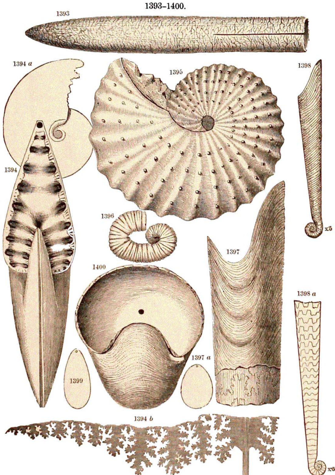
CEPHALOPODS. — Fig. 1393, Belemnitella Americana ; 1394, a, b , Placenticeras ( Ammonites ) placenta ; 1395, Scaphites Conradi ; 1396, S. larvæformis ; 1397, 1397 a , Baculites ovatus ; 1398, young stage of B. compressus ; 1398 a , same, with outer layer of shell removed, showing sutures; 1399, section of B. compressus , reduced; 1400, Nautilus Dekayi . Figs. 1393-1397, 1399, 1400, Meek; 1398, 1398 a , A. P. Brown.
