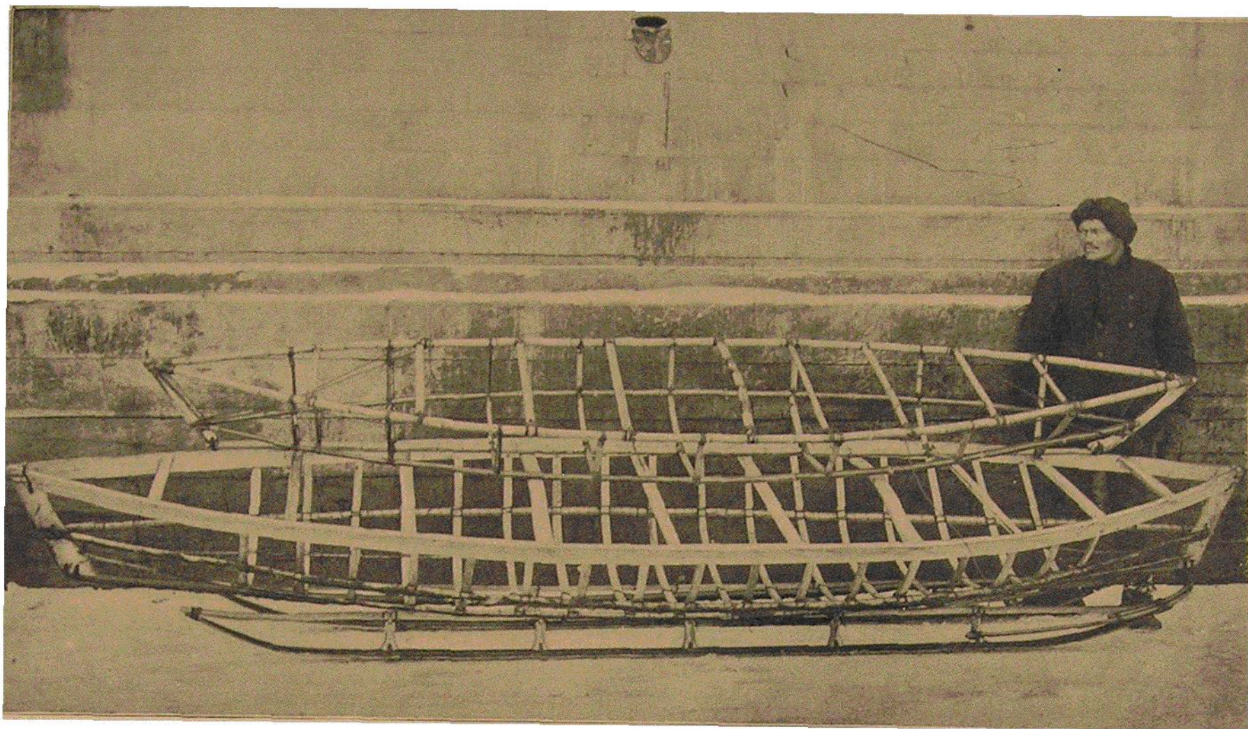
SKELETONS OF A KAYAK FOR ONE MAN (BAMBOO) AND OF A DOUBLE KAYAK, LYING ON A HAND-SLEDGE (From a photograph)
