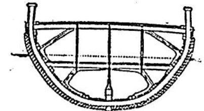
Fig. 3. Transverse section amidships.
