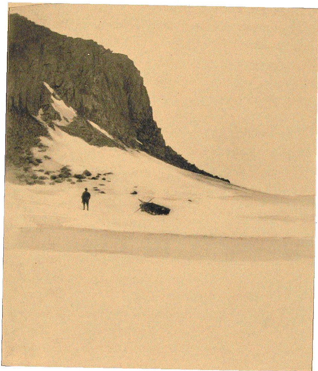
BASALTIC CLIFFS
