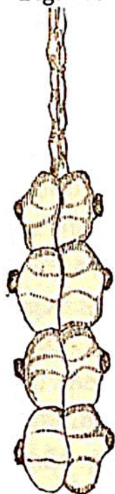
Cephalitis Bowdichii.
