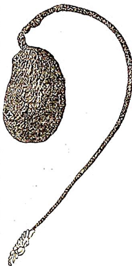
Boltenia.
