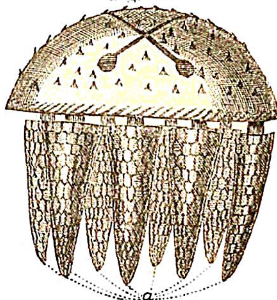
Cephea mosaica .
