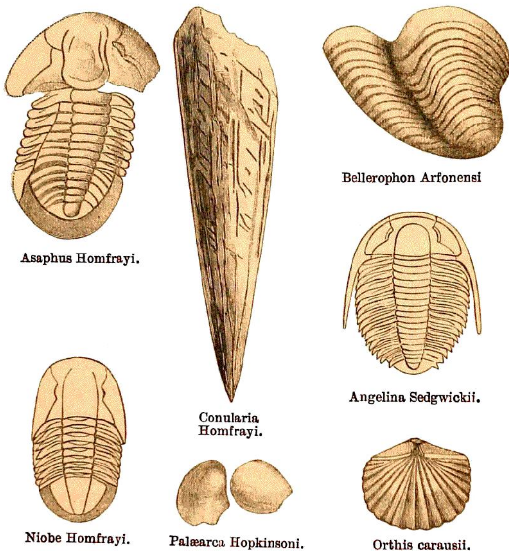
Group of Tremadoc Slate Fossils.
