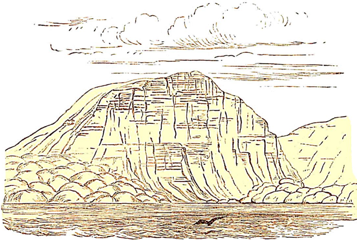
Fig. 21.—Ben Shieldag, Loch Torridon—a hill of flat Cambrian red sandstone resting upon an uneven hummocky surface of the old gneiss.
