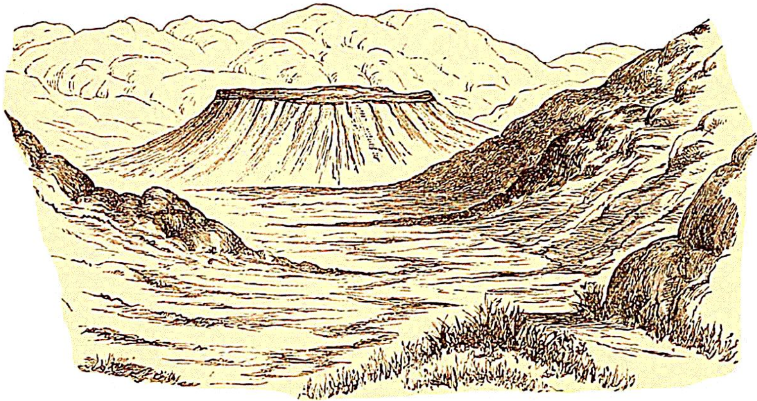
Fig. 22.—View of outlier of Cambrian breccia and sandstone among gneiss hills, near Gairloch.
