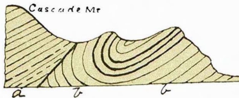
FIG. 1. DIAGRAM ILLUSTRATING FOLDING OF THE CRUST OF THE EARTH.—(a) Undisturbed crust. (b) Primary depression and deposition. (c) Mountain-making folds with their relations to an upper and lower magma. Fig. 2. Result of folding, faulting, and denudation, as seen at Cascade Mountain, Western Canada (after McConnell, p. 33).
