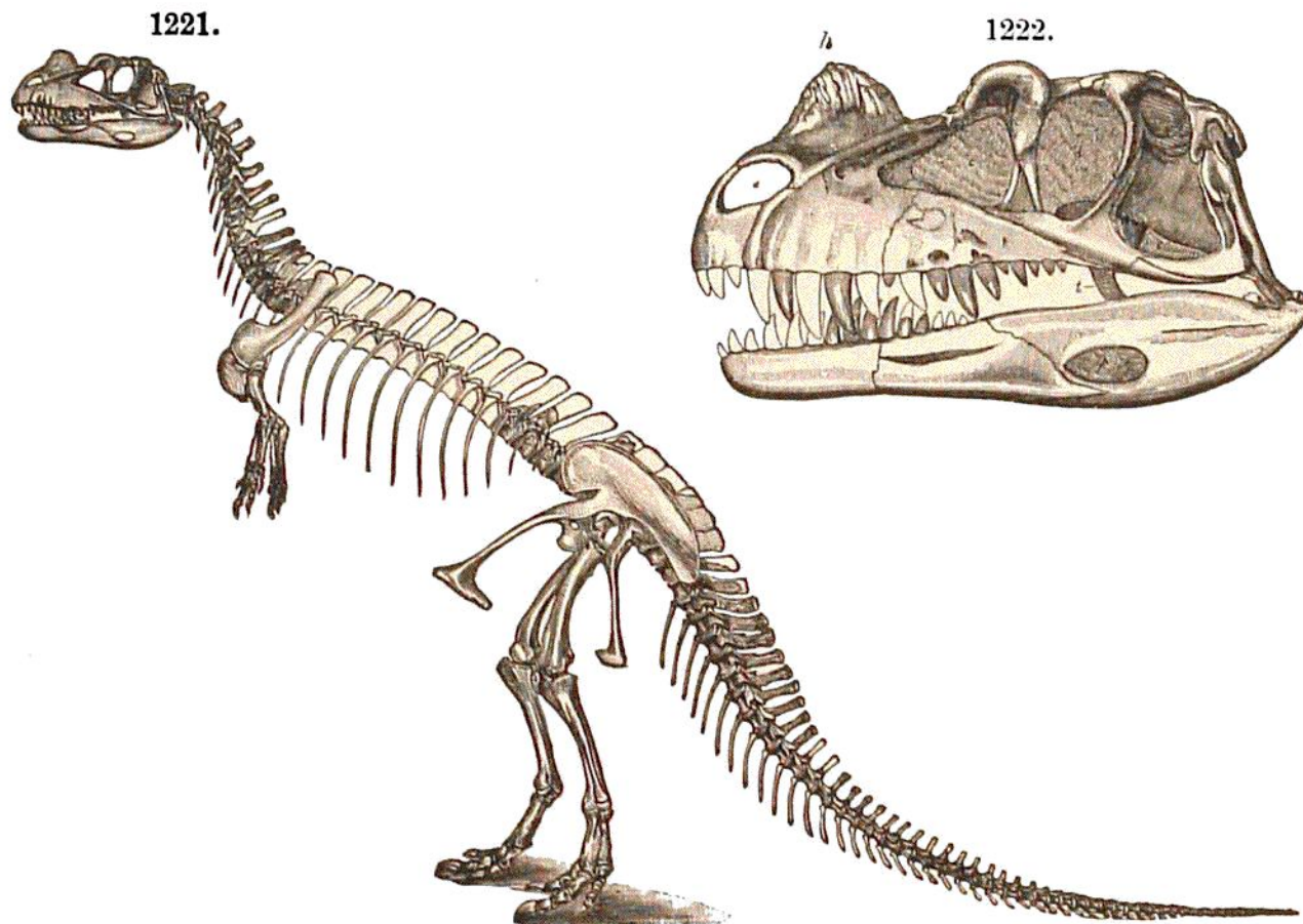
DINOSAUR. — Fig. 1221, Restoration of Ceratosaurus nasicornis ( \times \frac{1}{20} ); 1222, skull of same ( \times \frac{1}{10} ); h , horncore. Marsh.
