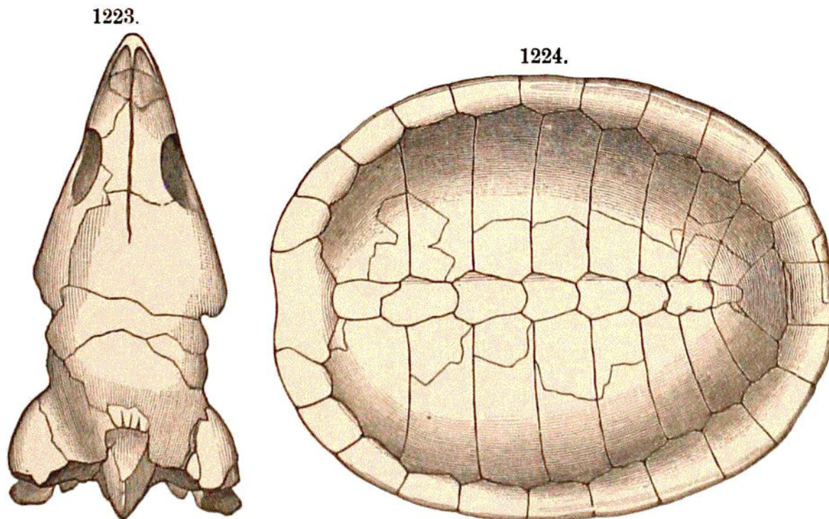
TURTLES. — Fig. 1223, Glyptops , a Turtle skull, natural size; 1224, carapace of probably the same species ( \times \frac{1}{2} ). Marsh.
