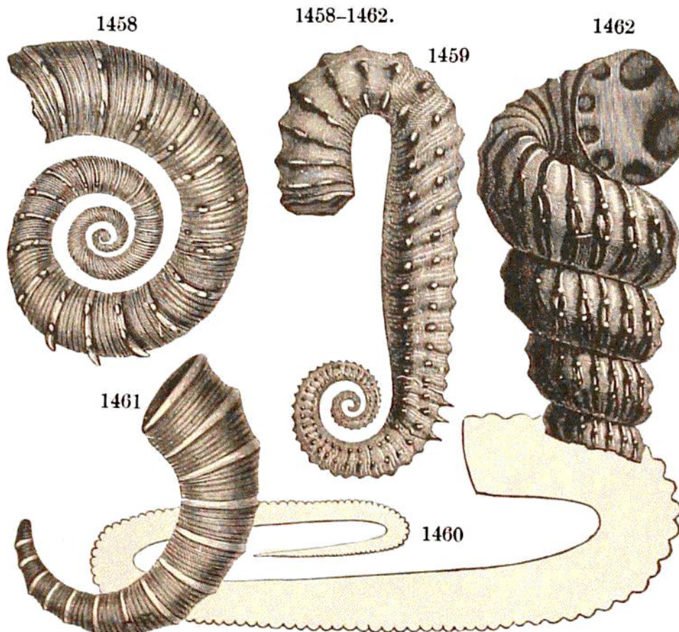
CEPHALOPODS, Ammonite Family. — Fig. 1458, Crioceras Duvallii ; 1459, Ancyloceras Matheronianum , 1460, Hamites attenuatus ; 1461, Toxoceras bituberculatum ; 1462, Turrillites catenatus .
