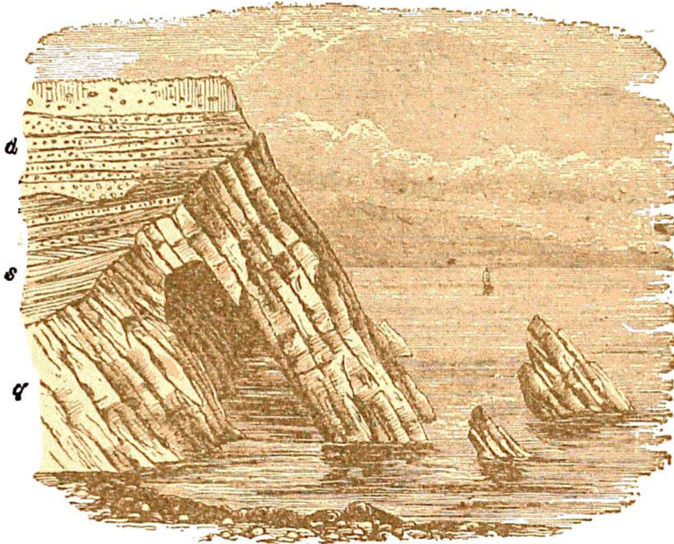
Fig. 325.—Double Unconformability at Cullen, Banffshire. q , Quartzite; s , Old Red Sandstone; d , Post-Tertiary Gravels.
